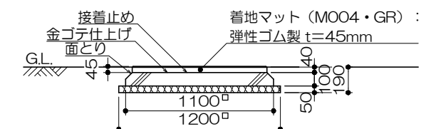
D型基礎x1ヶ
